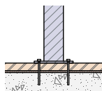
Bolt Through
